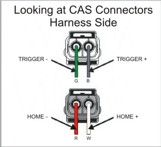
Figure 15- 3 rd Generation Crank Angle Sensor Location and wiring
