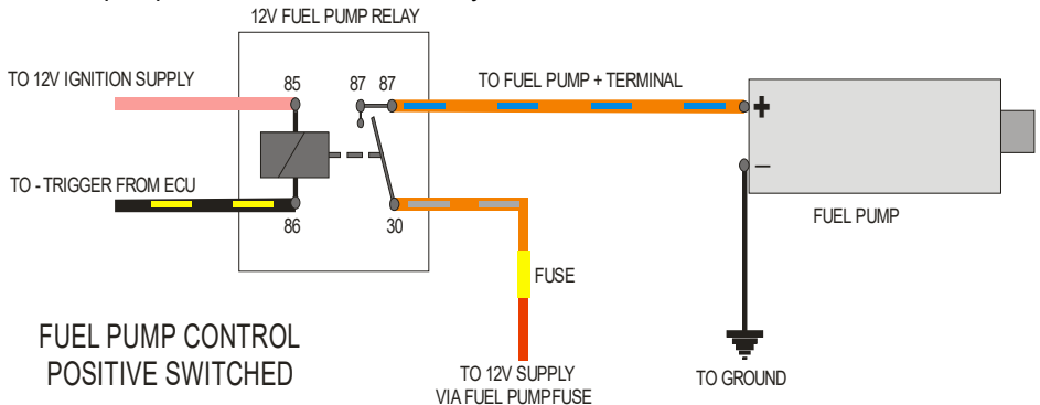
Figure 6- Fuel Pump Wiring
