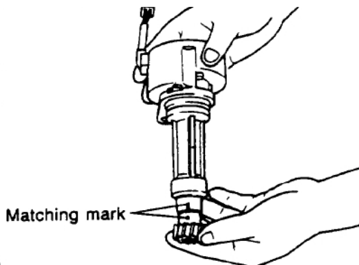
Figure 11- Crank Angle Sensor Alignment with Drive Gear
