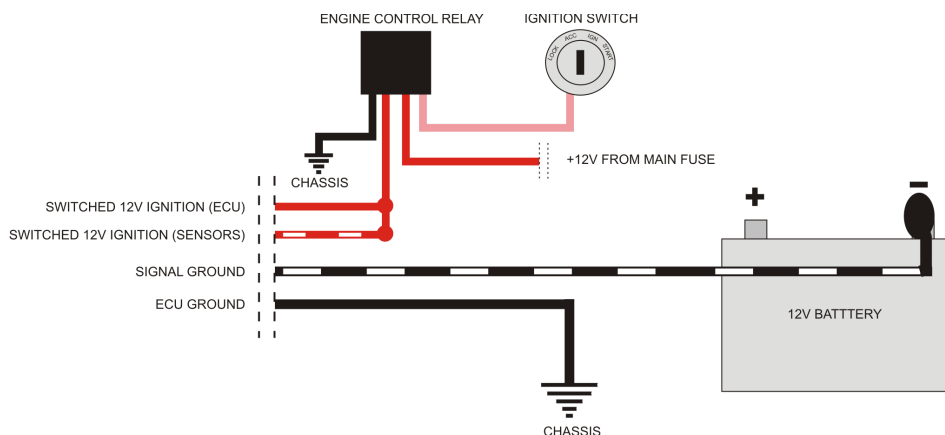
Figure 9 – Main Power Wiring
