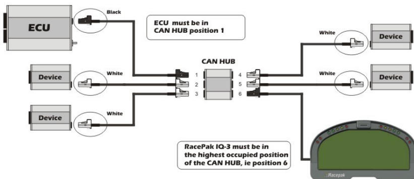
Figure 24 – Haltech ECU connected to 5 Auxiliary CAN based devices
