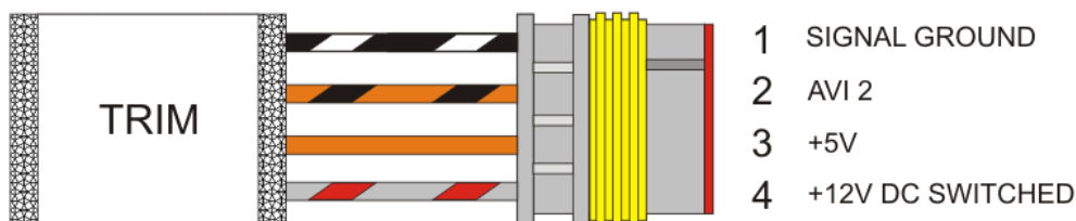
Figure 7- Trim Module Connector Pinout
