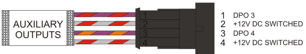
Figure 3 - Auxiliary Output Connector
