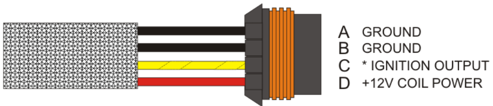
Figure 9 – Haltech LS1 Ignition Harness Connections
