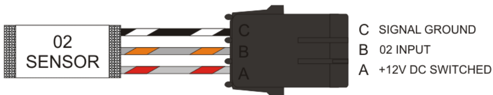
Figure 4 - 02 Sensor Connector
