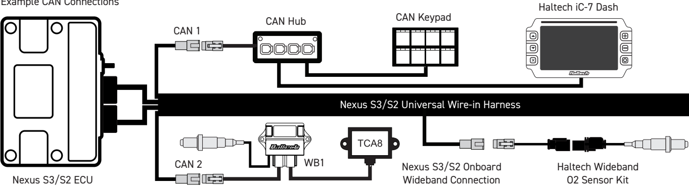
Example CAN Connections
