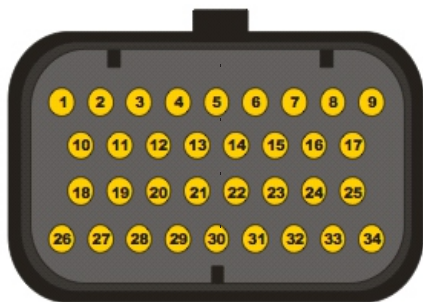
(34 Pin Connector)
