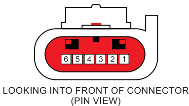
Figure 4 - Electronic Throttle Body Wiring
