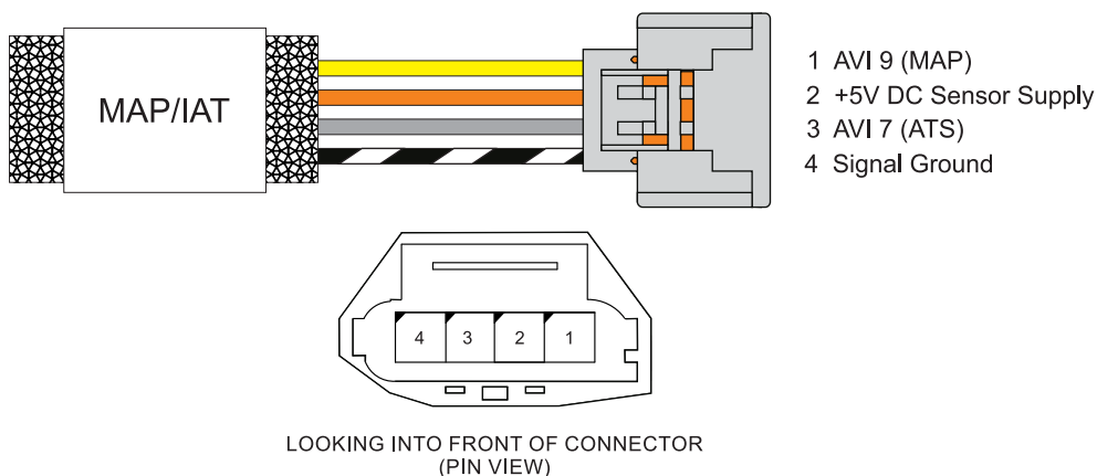
Figure 3 - MAP and IAT Wiring
