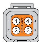
LOOKING INTO REAR OF CONNECTOR (HARNESS VIEW)
