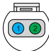
CAS (HOME) CONNECTOR PINOUT HARNESS SIDE VIEW
