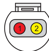
CAS (TRIGGER) CONNECTOR PINOUT HARNESS SIDE VIEW
