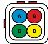
CAS SIDE CONNECTOR PINOUT HARNESS SIDE VIEW
