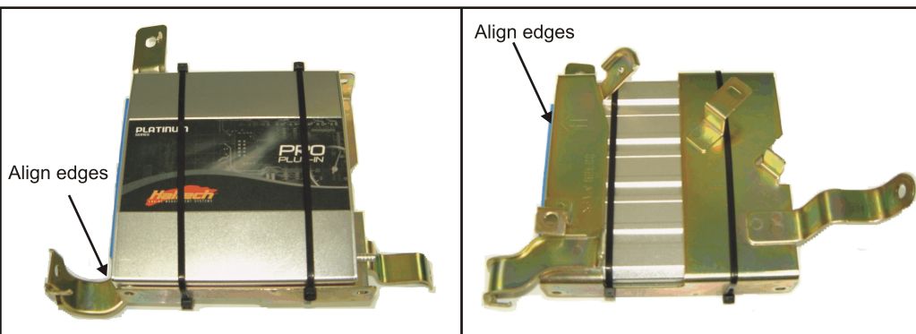
Figure 3 – Haltech ECU Mounted to Factory ECU Mount
