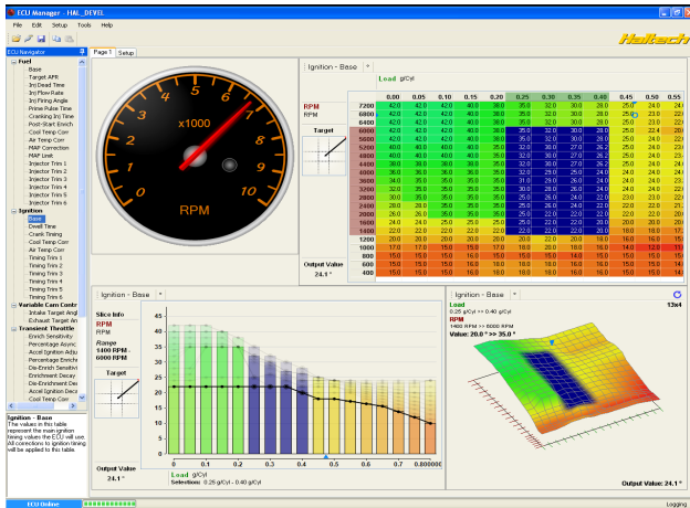
Figure 6 – Haltech ECU Manager Software tuning page
