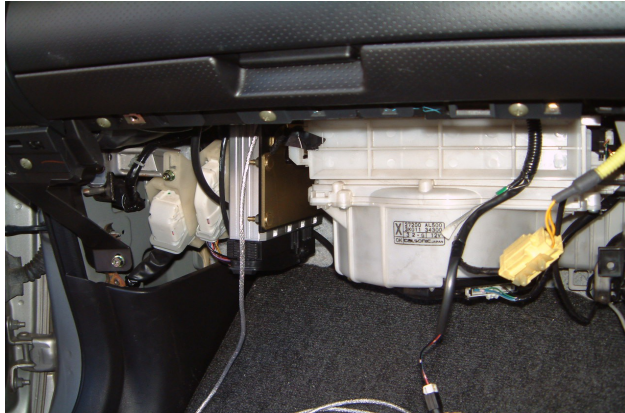
Figure 5 – Haltech ECU Installed in OEM Location
