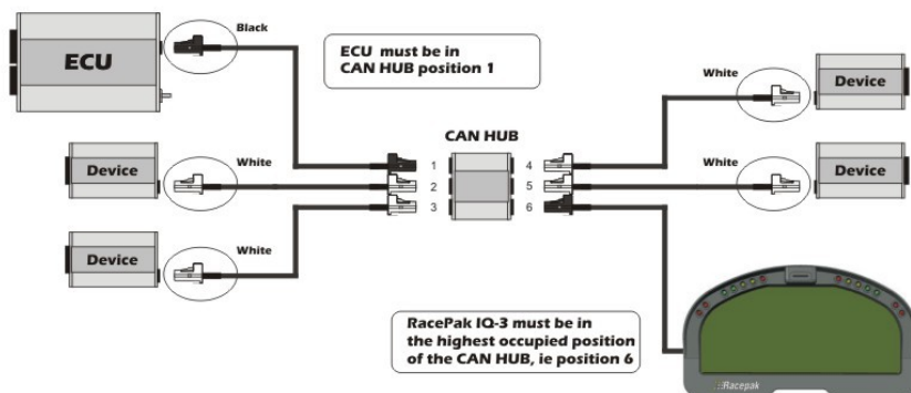
Figure 15 – Haltech ECU connected to a Racepak Dash
