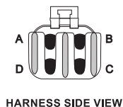
HARNESS SIDE VIEW
