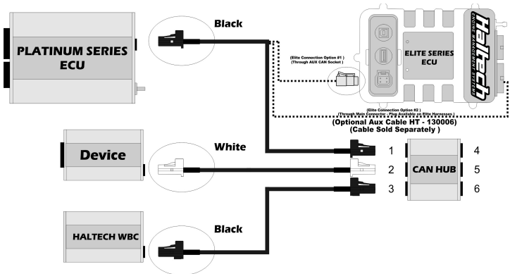
Figure 2 – Haltech CAN Wideband Controller connected via the Haltech Can Hub
