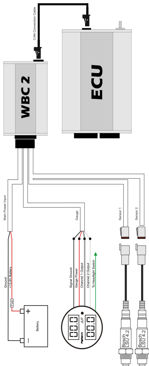
Figure 14 – Haltech WBC 2 Installation Diagram (CAN)
