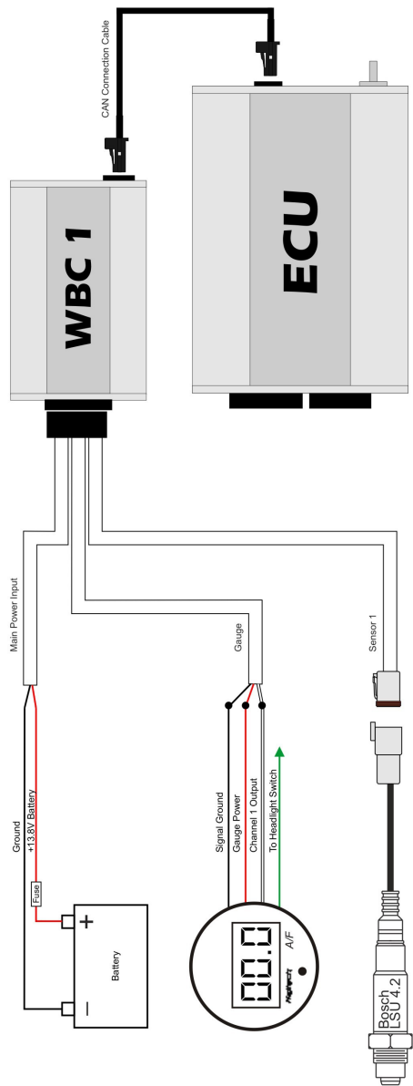
Figure 13 – Haltech WBC 1 Installation Diagram (CAN)
